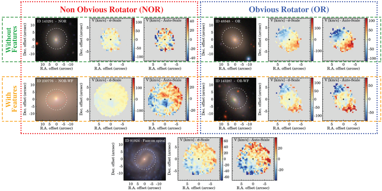
Figure 5. Example velocity maps and gri VST-KiDS or Subaru-HSC colour images for Non-Obvious Rotators (left) versus Obvious Rotators (right), and Face-on Spirals (bottom) as used in the SAMI Galaxy Survey kinematic visual classification. The white-dashed circle on the images shows the SAMI field-of-view, whereas the blue- or red-dashed ellipse on the velocity maps respectively shows 1R_e or 0.5R_e . For each galaxy, the first velocity map is used to classify galaxies into NORs and ORs. Here, the velocity scale is derived from the velocity dispersion \pm\sigma_e . This integrates the velocity dispersion into the visual classification such that with increasing velocity dispersion the rotational velocity has to become more pronounced in order for a galaxy to be classified as an obvious rotator. The auto-scaled velocity map is included to aid classifiers in identifying kinematic substructures (WF).
