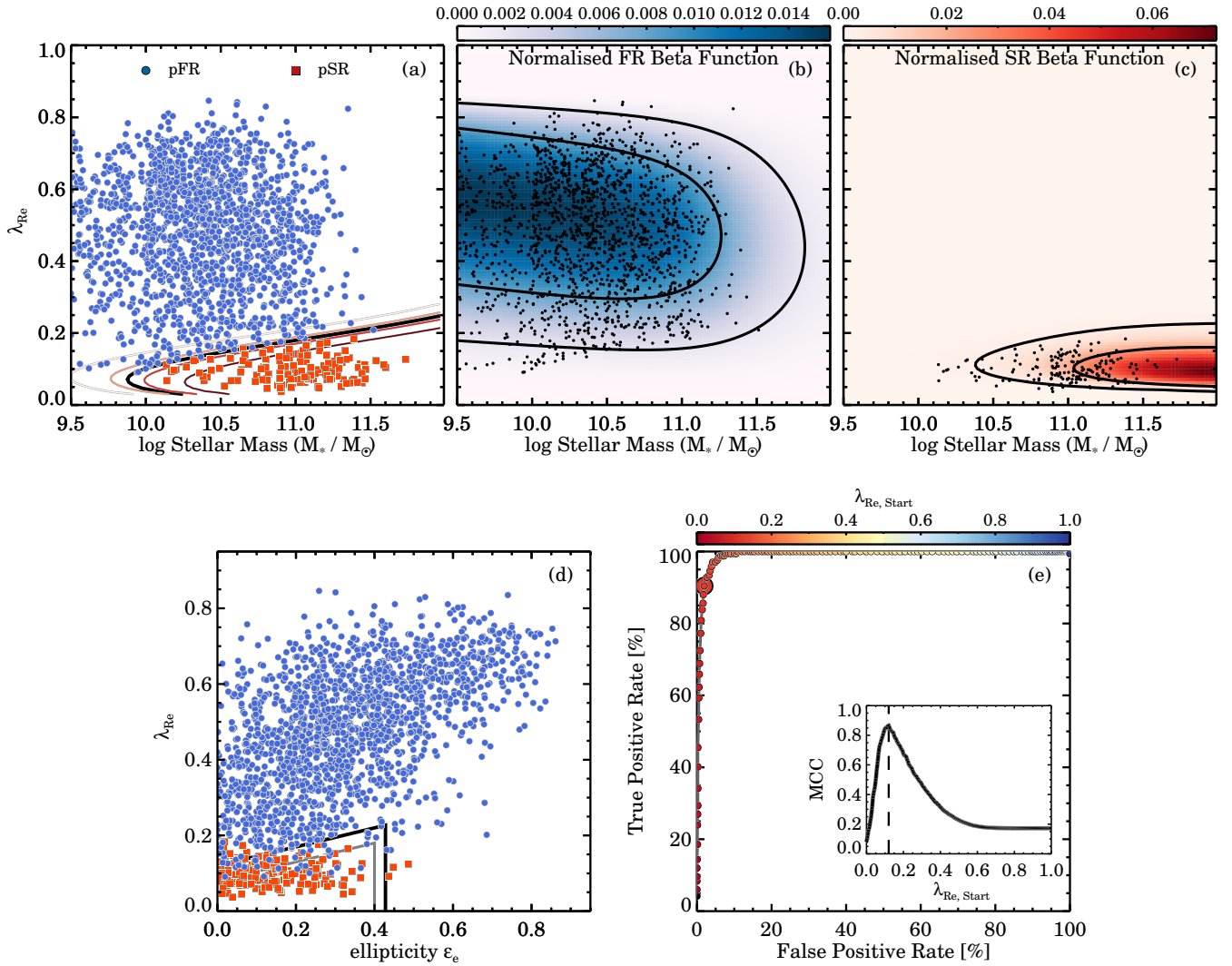
Figure 9. Seeing-corrected spin parameter proxy versus stellar mass and ellipticity. We present the probabilistic Fast and Slow rotators (pFRs and pSRs) as blue and red coloured symbols in panel (a), with contours marking the probability for a galaxy to be a slow rotator (p(SR)=50% black, and from light to dark red as 20%, 40%, 60%, 80%). Panels (b) and (c) show the fast and slow rotator PDFs normalised in each mass bin, with contours enclosing 68 and 95 percent of the PDF, and indicates the probability of finding a pSR or pFR if the mass-function is flat. The SAMI classified pFRs and pSRs are shown in the \lambda_{Re} - \epsilon_e space in panel (d) where the optimal selection region from our ROC analysis is shown in black together with the Cappellari (2016) SR selection box in grey. Because we select pFRs and pSRs from the p(SR)=50% contour in the \lambda_{Re} - \log(M_\star/M_\odot) , the small increase of the \lambda_{Re} limit with stellar mass results in some minor contamination in the \lambda_{Re} - \epsilon_e space. Nonetheless, panel (e) indicates an extremely high True Positive Rate with low False Positive Rate, but this is partly by construction.
