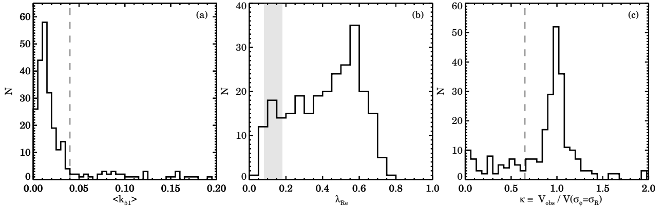
Figure C1. Distributions of \langle k_{51,e} \rangle , \lambda_{Re} and \kappa from the ATLAS 3D survey. The vertical lines in panel (a) and (c) indicate the proposed division for regular and non-regular rotators (panel a) and slow and fast rotators using JAM modelling panel (c), whereas the wider gray region in panel (b) indicates the Cappellari (2016) FR/SR selection region that includes an ellipticity term.
