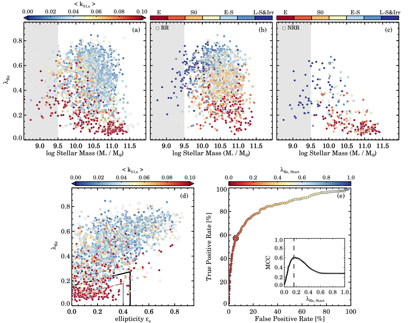
Figure 4. Seeing-corrected spin parameter proxy versus stellar mass and ellipticity. Data are colour coded by the kinematic asymmetry parameter \langle k_{51,e} \rangle (panel a) and visual morphological type (panels b and c). Unfilled symbols indicate that \langle k_{51,e} \rangle could not be measured within one R_e , or a conclusive visual morphology could not be determined. Galaxies below \log(M_*/M_\odot) < 9.5 are not used in the main analysis, but are shown here for completeness. The overlap of RRs and NRRs increases towards lower stellar mass. The low-mass NRRs also have higher values of \lambda_{R_e} as compared to high mass NRRs. We show the RRs and NRRs in the \lambda_{R_e} - \varepsilon_e space in panel (d) with the optimal selection region (black) derived from panel (e) and the slow rotator selection box from Cappellari (2016) in grey. There is considerable overlap of RR and NRR rotators. Panel (e) shows the "Receiver Operating Characteristic Curve" and Matthews correlation coefficient distribution from which we derive the optimal selection region. The most optimal selection region has a True Positive Rate of only 57.4 percent with a False positive rate of 5.7 percent. This suggests that the \lambda_{R_e} - \varepsilon_e space is not ideal for distinguishing between regular and non-regular rotators derived from SAMI data.
