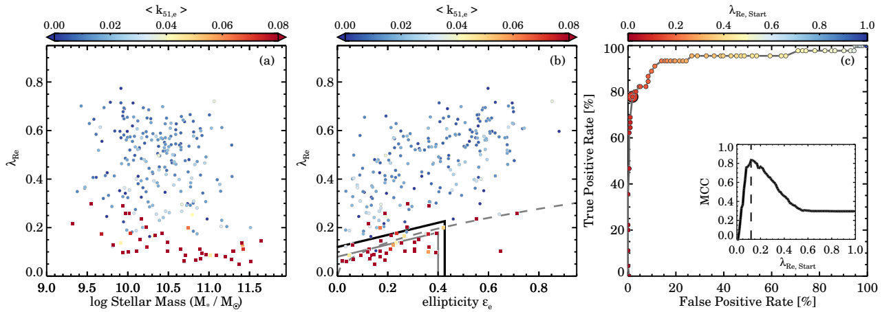
Figure D1. Spin parameter proxy versus stellar mass and ellipticity using ATLAS 3D data. Data are colour coded by \langle k_{51,e} \rangle (panels a and b). Round symbols show Regular Rotators, and diamond symbols. We show the RRs and NRRs in the \lambda_{Re} - \epsilon_e space in panel (b) with the optimal selection region (black), the SR selection box from Cappellari (2016) in grey, and from Emsellem et al. (2011) as the dashed line. Panel (c) suggests that the \lambda_{Re} - \epsilon_e space is an effective way to distinguishing between regular and non-regular rotators derived from ATLAS 3D data.
