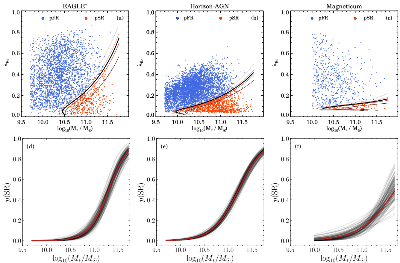
Figure 10. Bayesian mixture model analysis to identify different kinematic populations in the EAGLE + (left), HORIZON-AGN (middle), and MAGNETICUM (right) simulation using the spin parameter proxy versus stellar mass. The probabilistic fast and slow rotators (pFRs and pSRs) are shown as blue and red coloured symbols. The contours mark the probability for a galaxy to be a slow rotator (p(SR)=50% black, and from light to dark red as 20%, 40%, 60%, 80%). We find that the pSR/pFR divide in HORIZON-AGN closest matches the observations, whereas the EAGLE + and MAGNETICUM pSR/pFR cutoff reveal a respectively stronger and milder increase of the pSR distribution as a function of stellar mass.
