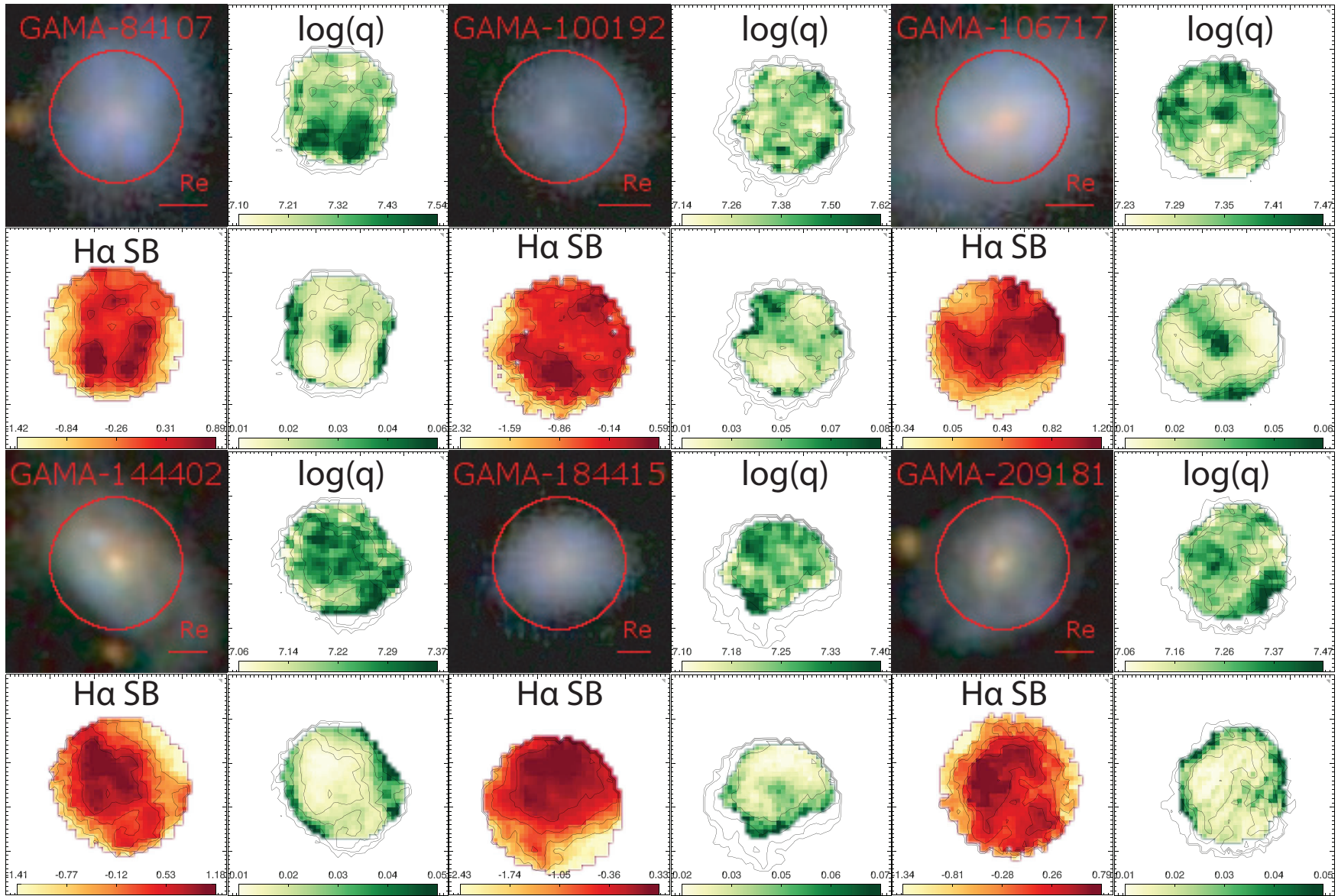
Figure B1. Same as Figure 8 for GAMA-84107, GAMA-100192, GAMA-106717, GAMA-144402, GAMA-184415 and GAMA-209181.
