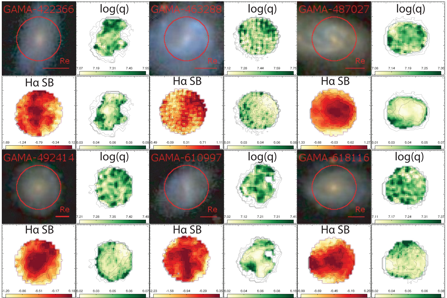
Figure B3. Same as Figure 8 for GAMA-422366, GAMA-463288, GAMA-487027, GAMA-492414, GAMA-610997 and GAMA-618116.
