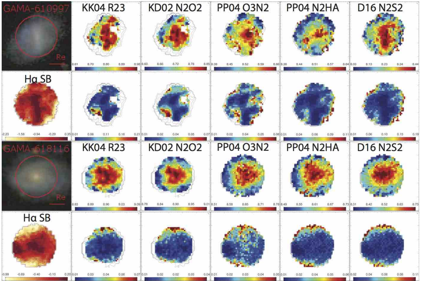
Figure A11. Same as Figure 2 for GAMA-610997 and GAMA-618116.
