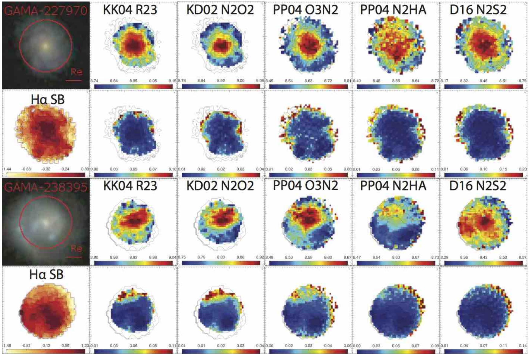
Figure A7. Same as Figure 2 for GAMA-227970 and GAMA-238395.
