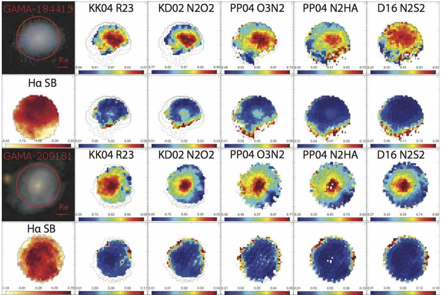
Figure A5. Same as Figure 2 for GAMA-184415 and GAMA-209181.
