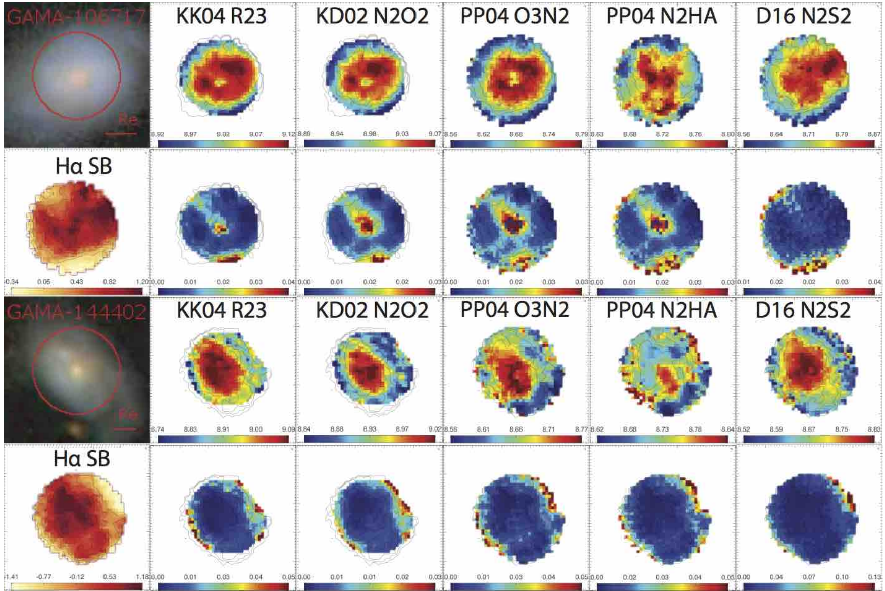
Figure A4. Same as Figure 2 for GAMA-106717 and GAMA-144402.
