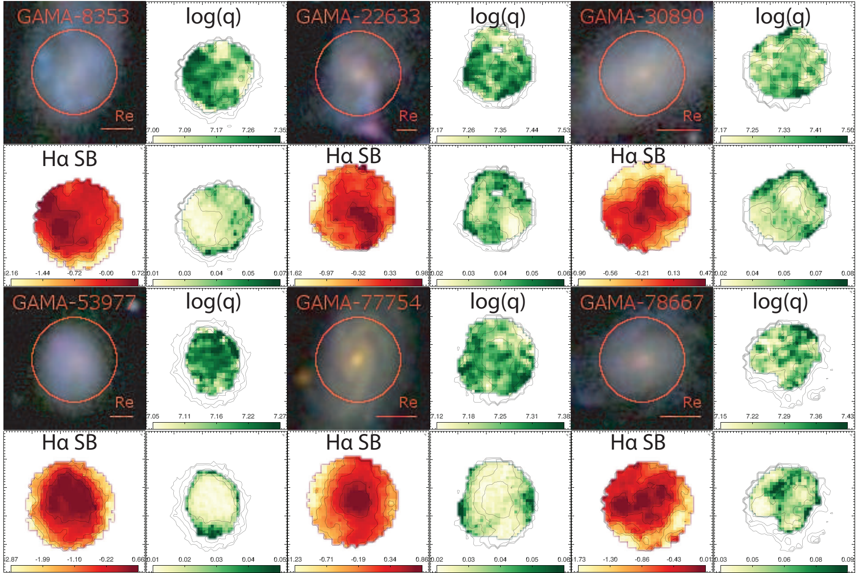
Figure 8. Each galaxy is presented with a 2 \times 2 grid containing the results of our work. The top left image of each grid contains the same SDSS image as Figure 2. The H\alpha emission line map with contours below the SDSS image is also identical to Figure 2. To the right of each SDSS image is the ionization parameter map in units of \log(\text{cm/s}) with overplotted H\alpha contours for comparison. Below each ionization parameter map is the associated error map as described in Section 3.6. Note that scale bars have been varied between different maps and galaxies in order to provide the best resolution possible
