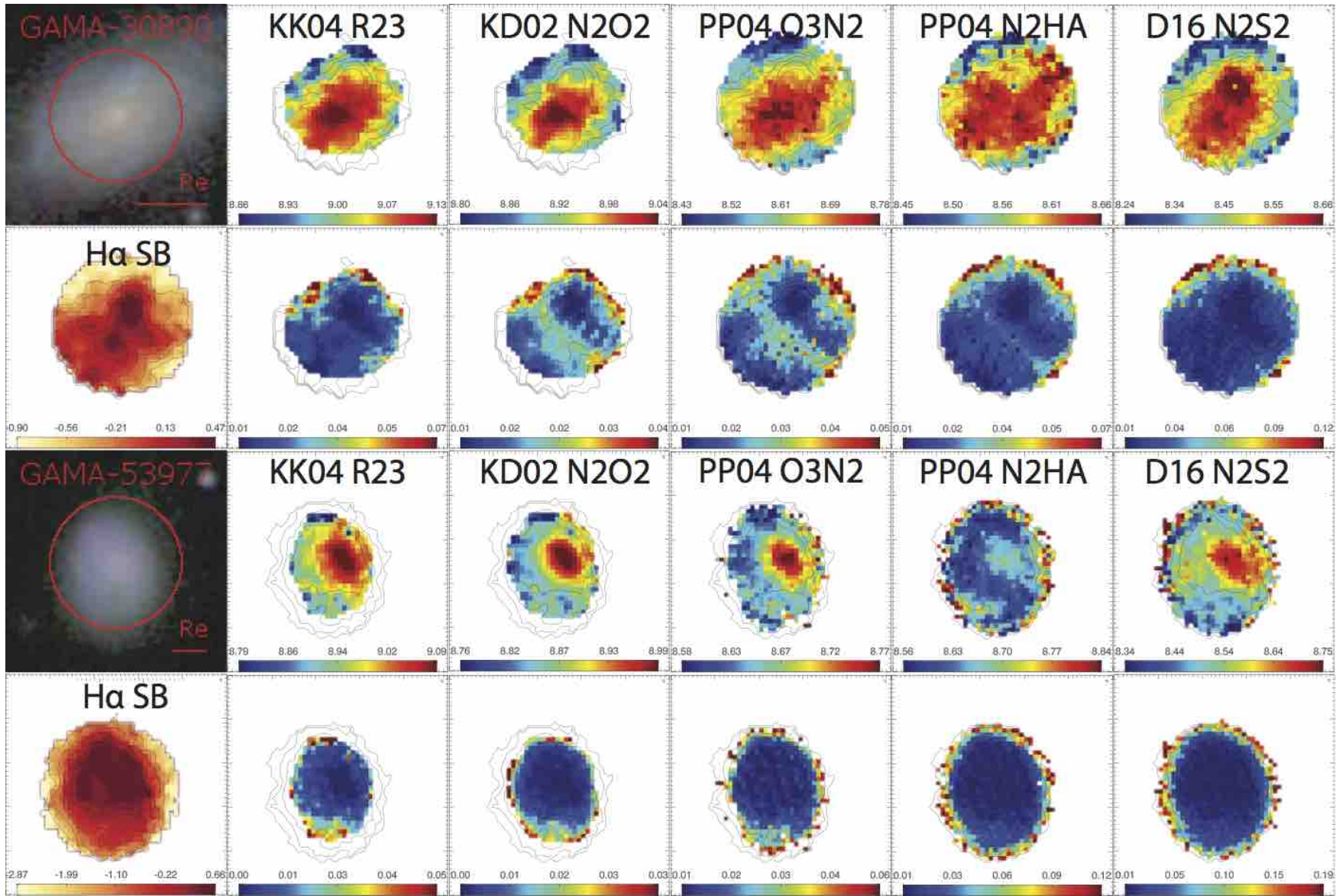
Figure A1. Same as Figure 2 for GAMA-30890 and GAMA-53977.
