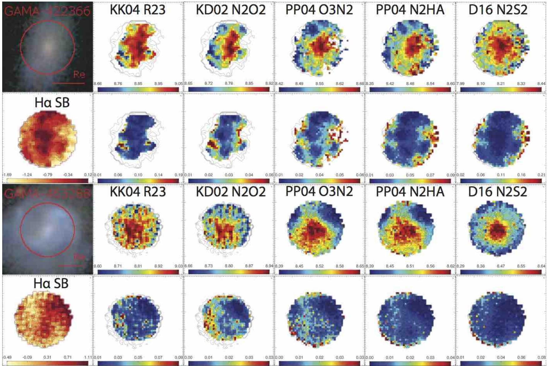
Figure A9. Same as Figure 2 for GAMA-422366 and GAMA-463288.
