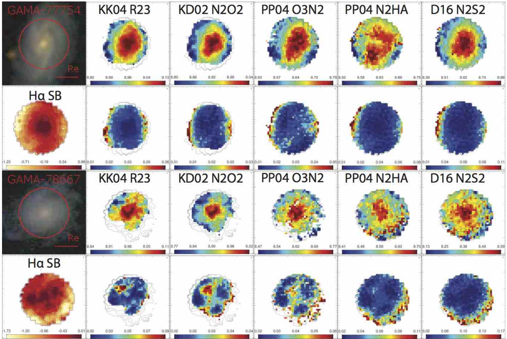
Figure A2. Same as Figure 2 for GAMA-77754 and GAMA-78667.
