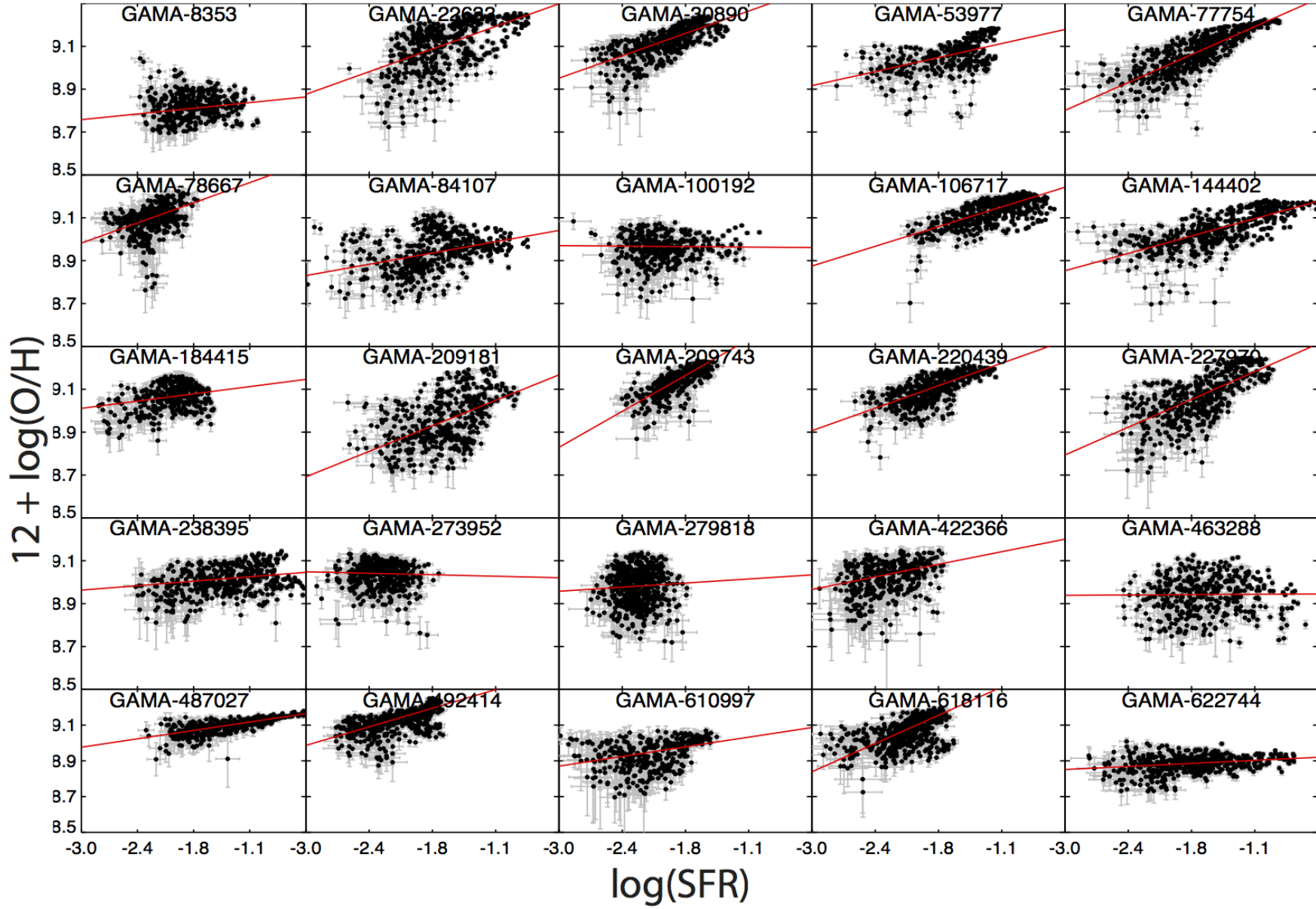
Figure 4. KK04 R_{23} metallicity as a function of SFR surface density. We obtain maps of SFR surface density in units of M_{\odot}/\text{year}/\text{kpc}^2 from Medling et al. (2018) . We show the best linear fit as a red line and summarise the results in the Table C1.
