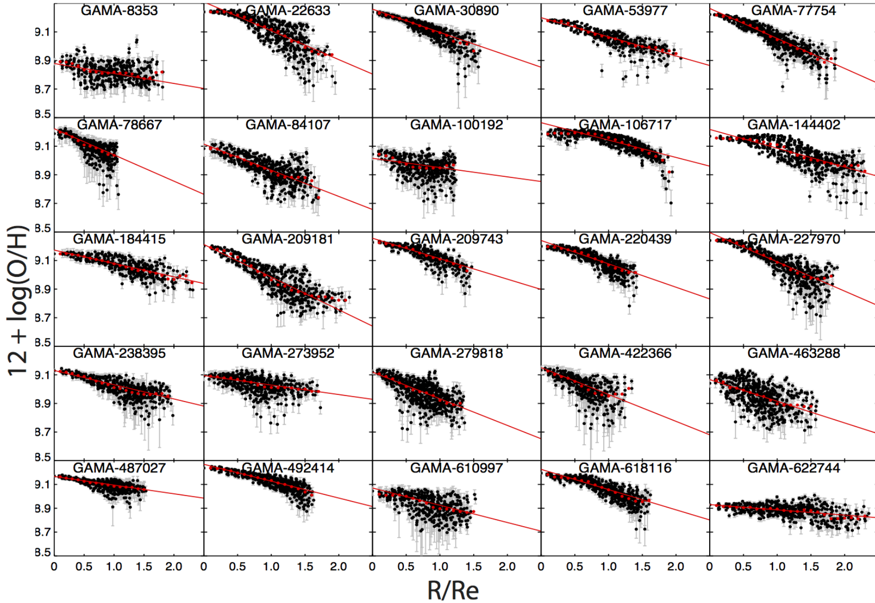
Figure 3. KK04 R_{23} metallicity gradients used in our analysis. We show 1\sigma error bars for each spaxel, determined from the method described in Section 3.6. The best linear fit to the metallicity gradient is given as a red line. The median metallicity in bins of 0.1 R/R_e are filled red circles. The results are summarised in Table 2.
