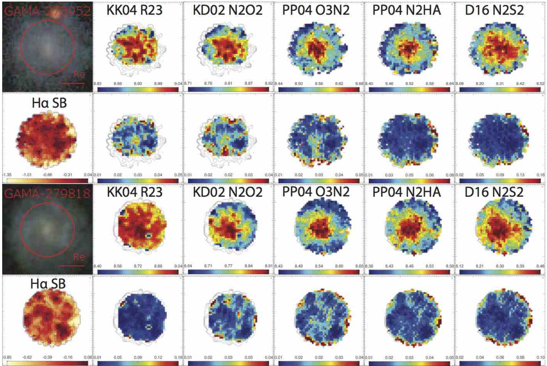
Figure A8. Same as Figure 2 for GAMA-273952 and GAMA-279818.
