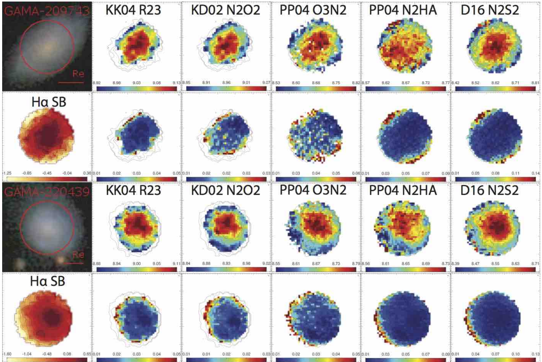
Figure A6. Same as Figure 2 for GAMA-209743 and GAMA-220439.
