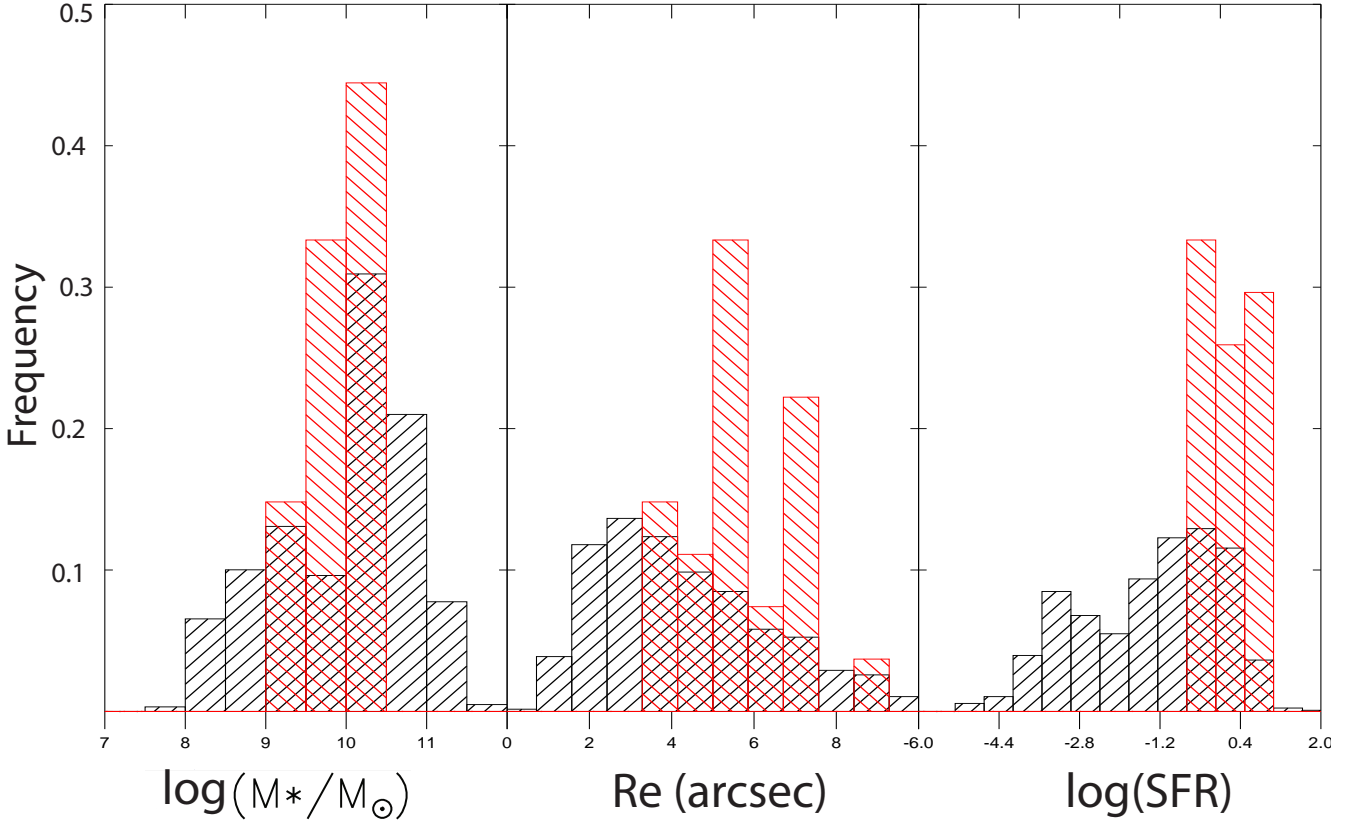
Figure 1. Comparison between DR1 of the SAMI Galaxy Survey (Black) and the final galaxy sample used for our analysis (Red). Left Panel: We have selected galaxies in the middle of the mass range ( 9.0 < \log M_*/M_\odot < 10.5 ) of DR1. Less massive galaxies are selected to have smaller redshifts and have comparable effective radii. This means that they are more diffuse and harder to obtain reliable S/N, leading to the lower mass limit. The upper mass limit is due to our restriction on sampling to at least 1R_e . As we are observing a fairly narrow redshift range, more massive galaxies tend to have a larger apparent size, meaning we are unable to achieve the minimum 1R_e we desire. Middle Panel: Again we sample the middle range of effective radii for the same reasons as we sample the middle range of stellar mass. The only exception is a slight spike beyond Re > 8'' . This comes from GAMA-422366, which has an ellipticity of 0.354, allowing it to be sampled beyond 1R_e along the minor axis despite the effective radius being larger than the SAMI field of view radius. Right Panel: Since we are aiming to only look at galaxies with high SFR fractions, we are only sampling the high SFR end of the DR1 SAMI Galaxy Survey.
