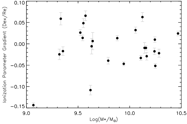
Figure 7. Normalized ionization parameter gradients using the KK04 O32 diagnostic as a function of stellar mass. We find no significant variation in the ionization parameter gradient as a function of galaxy mass.
