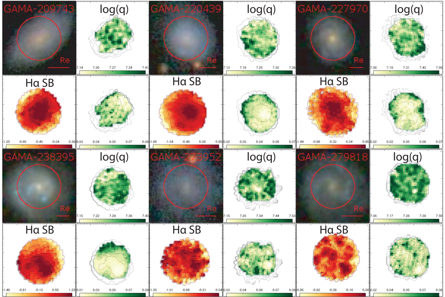
Figure B2. Same as Figure 8 for GAMA-209743, GAMA-220439, GAMA-227970, GAMA-238395, GAMA-273952 and GAMA-279818.
