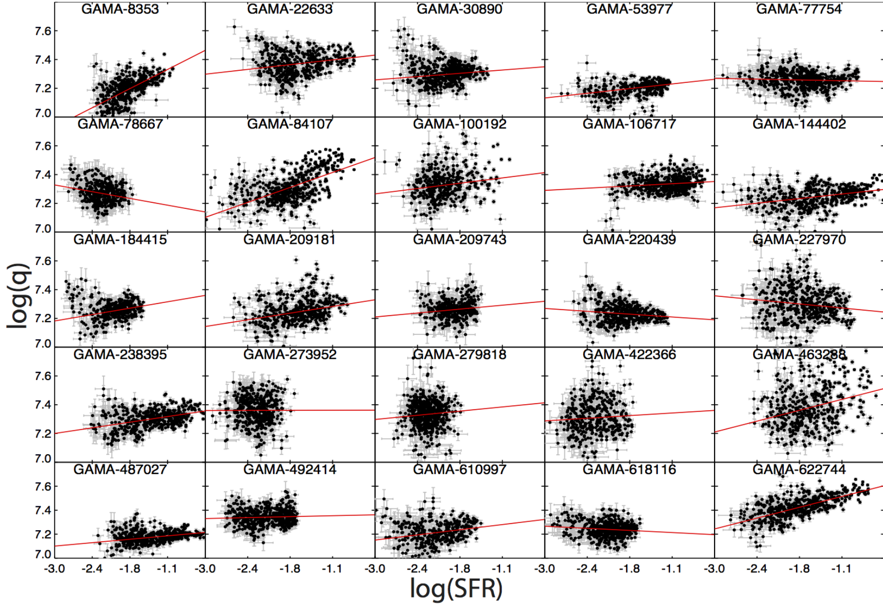
Figure 10. Same as Figure 4 for ionization parameter. We summarise the results in the Table C2.
