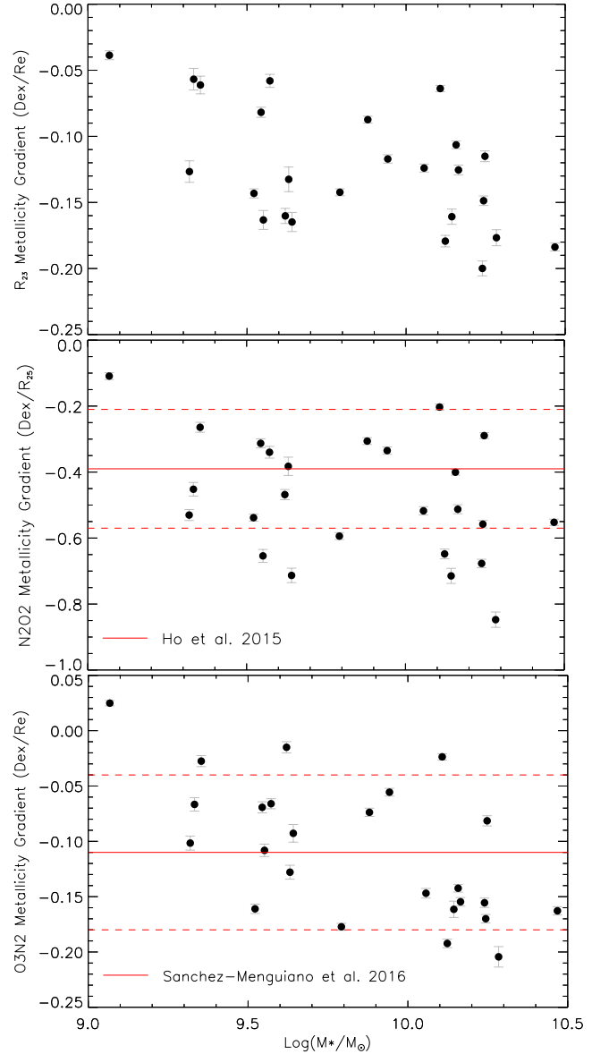
Figure 5. Normalised metallicity gradients as a function of mass using 3 common metallicity diagnostics. For the KD02 and PP04 metallicity diagnostics, we compare the results presented in Ho et al. (2015) and Sánchez-Menguiano et al. (2016a) . The solid red line show the mean metallicity gradient with 1\sigma scatter shown as dotted red lines.
