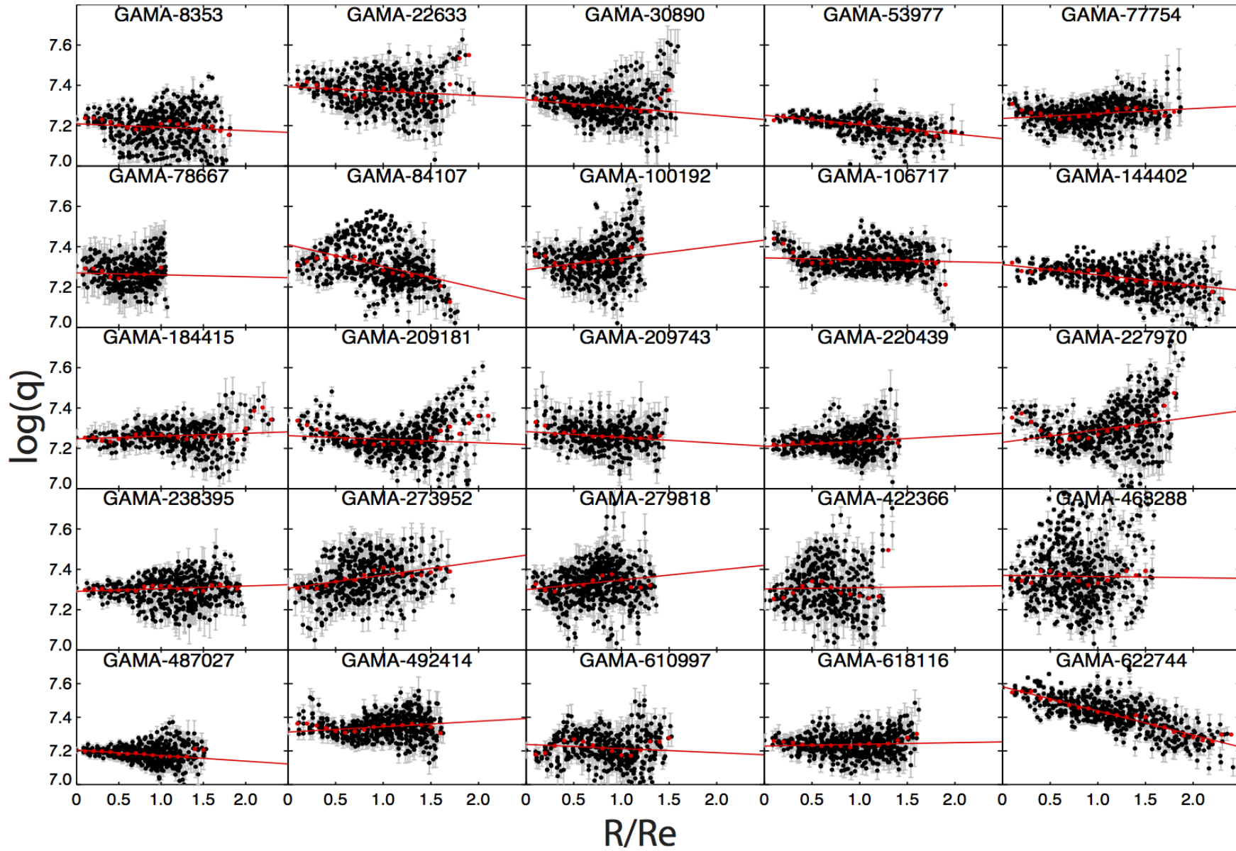
Figure 9. Same as Figure 3 for ionization parameter. The results are summarised in Table 3.
