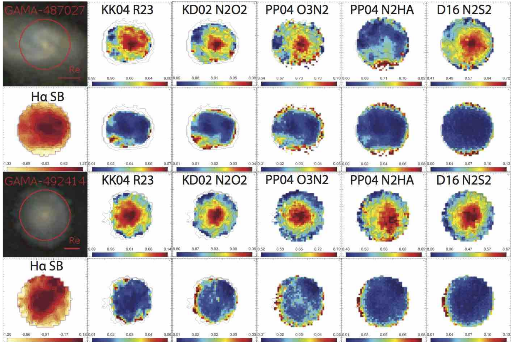
Figure A10. Same as Figure 2 for GAMA-487027 and GAMA-492414.
