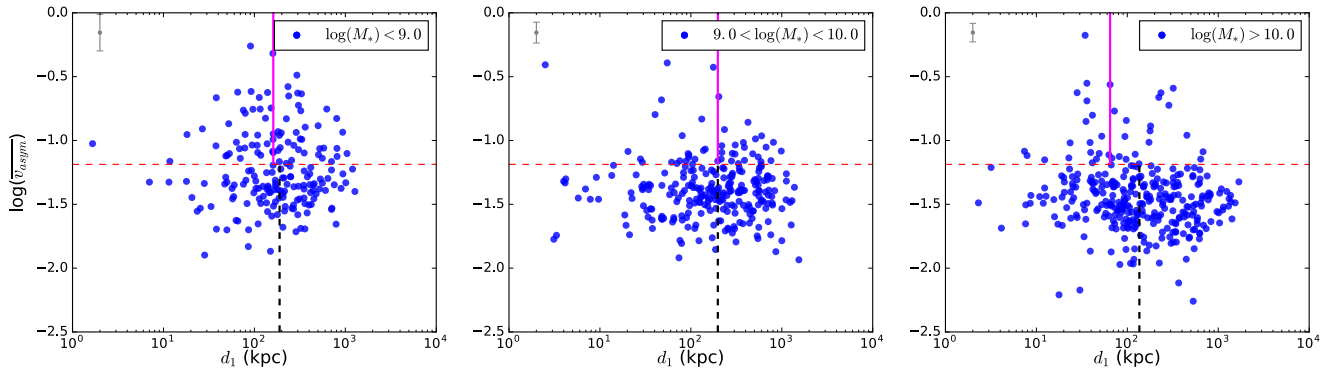
Figure 5. d_1 against \overline{v_{asym}} , in bins of stellar mass. There is a weak inverse correlation between d_1 and \overline{v_{asym}} for galaxies with \log(M_*/M_\odot) > 10.0 , but not for the two lower stellar mass bins. Low and high stellar mass galaxies also have different distributions of \overline{v_{asym}} and d_1 . Typical error bars are shown in grey (top left corner), and the \overline{v_{asym}} > 0.065 cutoff from Bloom et al. (2017) is shown in red (dashed). The median d_1 for galaxies with \overline{v_{asym}} > 0.065 (pink, 65 \pm 33 kpc) and \overline{v_{asym}} > 0.065 (black, dashed, 135 \pm 22 kpc) is shown for all three subsamples. There is a statistically significant offset of 71 \pm 39 kpc between these medians in the \log(M_*/M_\odot) > 10.0 sample, but not in the lower mass cases.
