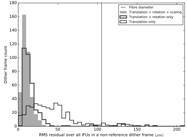
Figure 8. Histograms of the residuals after aligning dither frames. The alignment attempts to simultaneously place bundle centroids of all IFUs in a dither onto the centroids of the ‘reference’ dither frame. Distributions of residuals are shown for transformations with only a translation, a translation and a rotation, and the full transformation of a translation, a rotation, and a scaling.
