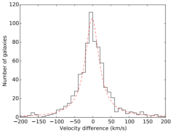
Figure 13. The distribution of rest-frame velocity differences between redshifted catalogued by GAMA and those from LZIFU for SAMI 1R_e aperture spectra, both corrected to the heliocentric reference frame. The red dashed line is a Lorentzian fit to the distribution.
