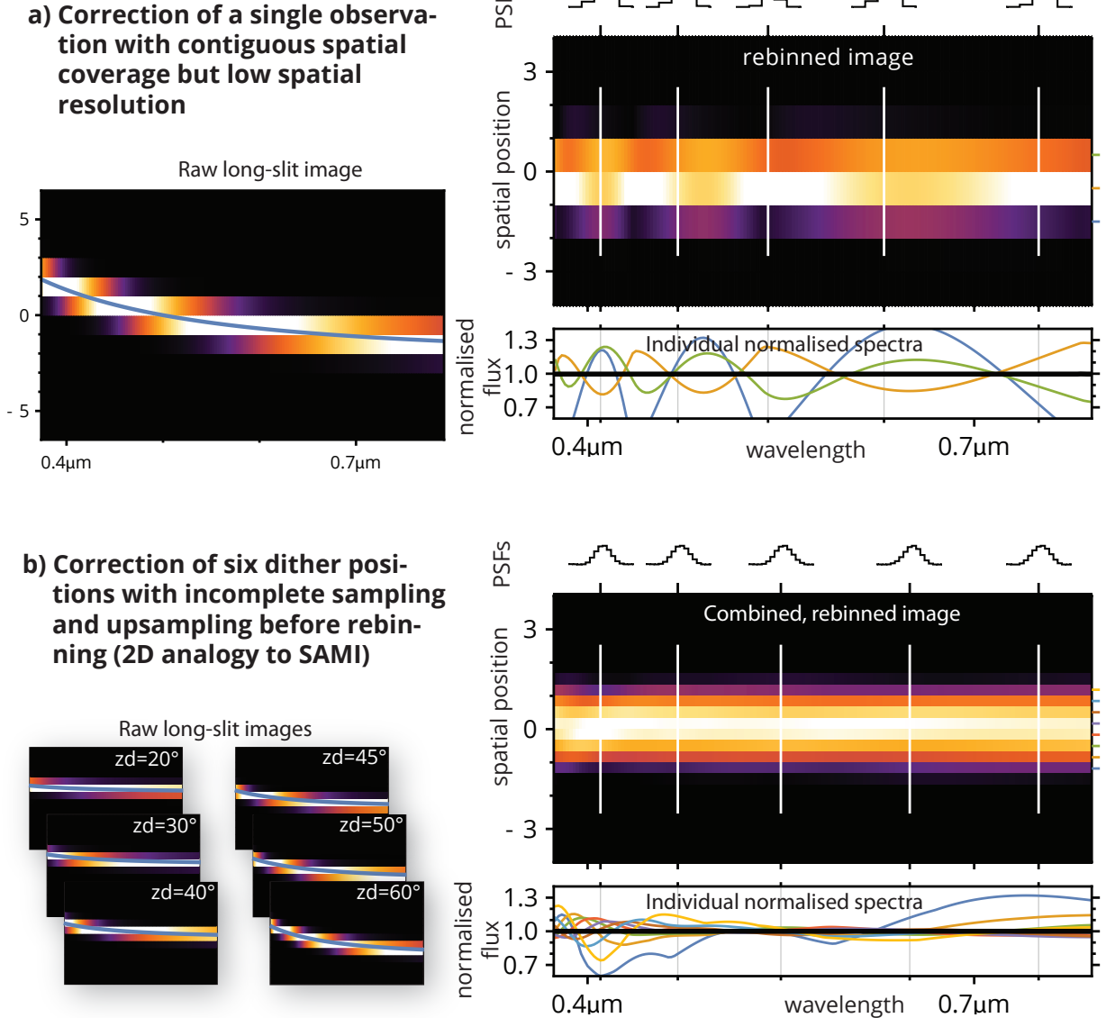
Figure 14. Long slit observations showing the effects of DAR and results of correcting for it in (a) a simple, single long-slit observation at high airmass, and (b) the combination of several long-slit observations at different air masses and dither positions—a close 2D analogy to our 3D data. The example shown in (a) is observed at a zenith distance of 60 degrees. The pixels are 1 arcsec, and the underlying Gaussian PSF has a FWHM of 1 arcsec. In (b), input frames are taken at six air-masses ranging from zenith distance (zd) of 20 to 60 degrees. The underlying PSF is the same, and the spatial pixels are also 1 arcsecond, but the spatial sampling is incomplete. In the rebinning to correct for DAR, the data are up-sampled to 0.33 arcsec pixels before combining.
