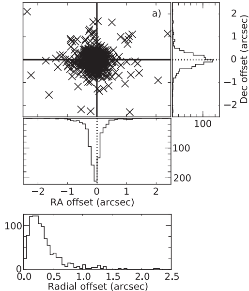
Figure 9. The difference between SAMI and SDSS astrometric solutions based on cross-correlation of images. (top) The distribution of RA and declination differences between SAMI and SDSS, with histograms of the differences in declination and right ascension along the axes. (bottom) Histogram of the distribution of differences in radial offset.
