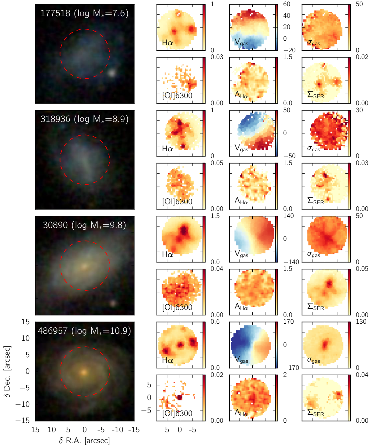
Figure 11. Examples of value-added products for four galaxies spanning the range of stellar masses included in our DR1. The red dashed circles on the SDSS 3-colour images (left) indicate the radius of the SAMI fibre bundle. The small panels show the various value-added products: H\alpha flux, gas velocity ( v_{gas} ), gas velocity dispersion ( \sigma_{gas} ), [O I]\lambda 6300 flux, H\alpha attenuation correction factor ( A_{H\alpha} ), and star-formation-rate-surface-density \Sigma_{SFR} maps. The units are 10^{-16} ergs s^{-1} cm^{-2} spaxel for the flux maps, km s^{-1} for the kinematic maps, magnitude for A_{H\alpha} , and M_{\odot} yr^{-1} kpc^{-2} for \Sigma_{SFR} .
