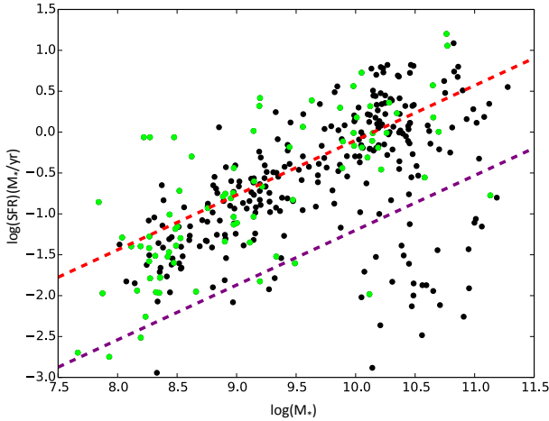
Figure 18. This figure shows SFR and stellar mass for normal galaxies (black) and kinematically identified asymmetric galaxies (green). We show the SFR main sequence from Noeske et al. (2007) (red dashed line), and the main sequence cutoff (purple dashed line). We see that asymmetric galaxies lie almost exclusively above the purple line, whereas normal galaxies are more evenly distributed.
