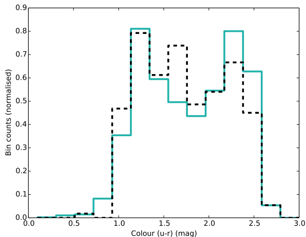
Figure 4. We show a normalised histogram of the colours in the SAMI Galaxy Survey sample (blue) and the sample used in this work (black, dashed). The data used were taken from the GAMA Data Release 2 catalogue SpecLineSFR (Hopkins et al. 2013).
