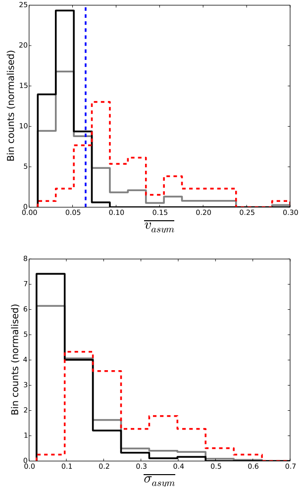
Figure 10. We show normalised histograms of \overline{v}_{asym} (top panel) and \overline{\sigma}_{asym} (bottom panel) for the whole sample (grey), visually classified normal (black) and asymmetric (red, dashed) galaxies. The cutoff value, \overline{v}_{asym} = 0.065 , is shown in blue.
