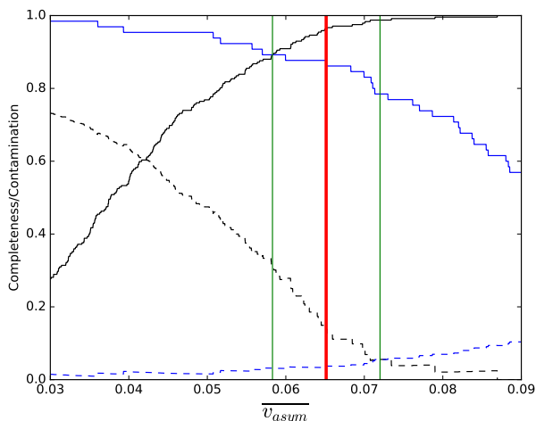
Figure 11. These curves show contamination (dashed) and completeness (solid) for visually asymmetric (blue) and visually normal (black) galaxies, at a range of values of v_{asym} . We choose our cut-off point (shown in red) as the midpoint between the points of intersection of the curves for contamination (number of visually normal galaxies classified as kinematically asymmetric and vice versa ) and completeness (number of visually asymmetric galaxies classified as kinematically asymmetric, similarly for visually normal galaxies) (shown in green). The points of intersection for contamination and completeness are 0.071 and 0.058, respectively, so we choose a cutoff value of \overline{v_{asym}} = 0.065 . See Section 4 for a complete explanation.
