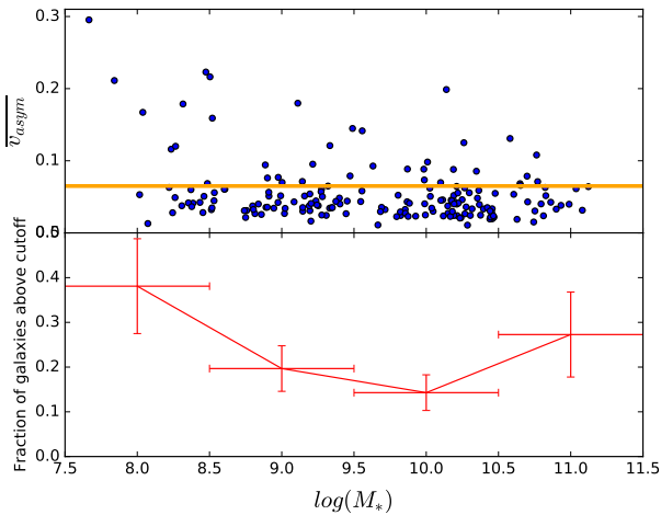
Figure 16. \overline{v_{asym}} is plotted against against stellar mass for the galaxies in our sample. The orange line shows our kinematic asymmetry cutoff, such that all galaxies above it are considered asymmetric. The bottom panel shows the fraction of galaxies, in bins of stellar mass (shown as horizontal error bars), above the asymmetry cutoff. This fraction decreases as a function of stellar mass.
