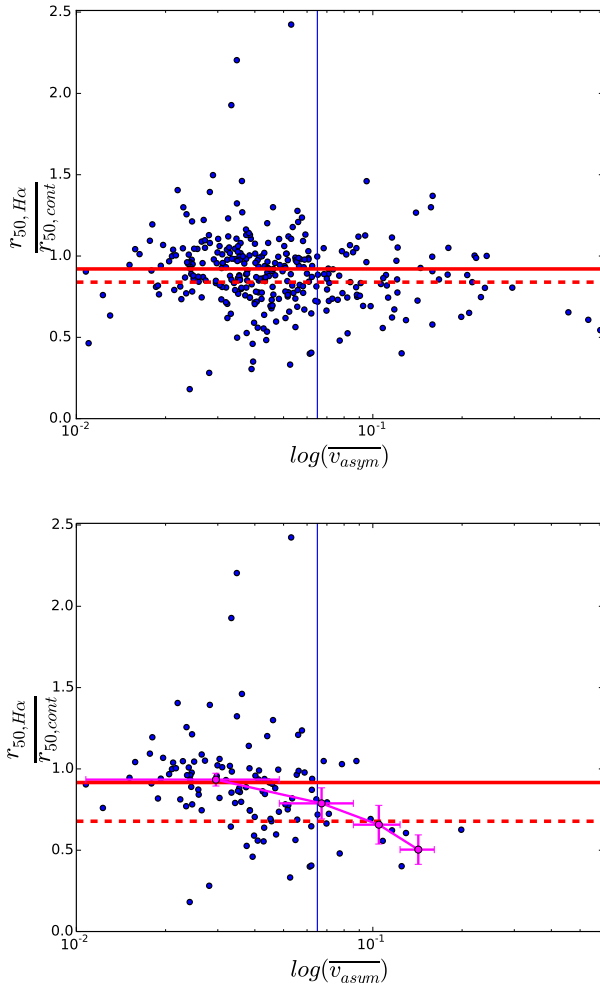
Figure 20. We show \log(\overline{v_{asym}}) against \frac{r_{50,H\alpha}}{r_{50,cont}} for all galaxies (top) and galaxies with \log(M_*) > 10.0 (bottom). The vertical blue line indicates the kinematic asymmetry cutoff \overline{v_{asym}} > 0.065 . Medians for normal (solid) and kinematically asymmetric (dashed) galaxies are shown in red. We see a 0.081 \pm 0.03 offset in median \frac{r_{50,H\alpha}}{r_{50,cont}} for all galaxies, and 0.27 \pm 0.07 offset for high mass galaxies, as well as an overall inverse correlation between \overline{v_{asym}} and \frac{r_{50,H\alpha}}{r_{50,cont}} in both cases. In the bottom panel, binned medians of \overline{v_{asym}} as a function of \frac{r_{50,H\alpha}}{r_{50,cont}} are shown in magenta, further demonstrating the downward trend. Vertical error bars show the error on the median, and horizontal bars show the extent of the bins in \log(\overline{v_{asym}}) .
