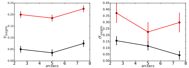
Figure 7. We show the values of v_{asym} (left) and \sigma_{asym} (right), with 1- \sigma errors, at the positions of the semi-major radii of the fitted ellipses for an asymmetric (red, GAMA618993) and non-asymmetric (black, GAMA567545) galaxy. It can clearly be seen that the velocity and velocity dispersion asymmetry values for the asymmetric galaxy are significantly higher than those of the normal galaxy. These are the same two galaxies shown in Fig. 6.
