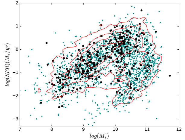
Figure 2. We show SFR against stellar mass for the GAMA Survey sample (log-spaced red contours), SAMI Galaxy Survey sample (blue points) and our sample (black dots). The \text{H}\alpha kinemetry sample has a slight bias against galaxies that fall off the main sequence of star formation, due to the cut in \text{H}\alpha S/N. The data used were taken from the GAMA Data Release 2 catalogues StellarMasses (Taylor et al. 2011) and SpecLineSFR (Hopkins et al. 2013).
