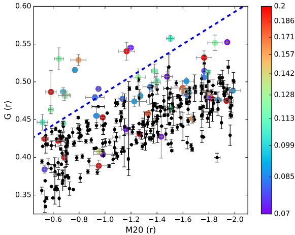
Figure 12. We show M_{20} against G , with kinematic classifications (normal galaxies in black, kinematically asymmetric galaxies in colour). We see that, even though the majority of galaxies falling above the line defined in Lotz et al. (2004) are kinematically asymmetric, there are many that would not be identified using this system. The colourbar shows the v_{asym} values on a log scale for the kinematically asymmetric points. We see that many of the most kinematically asymmetric points fall below the line.
