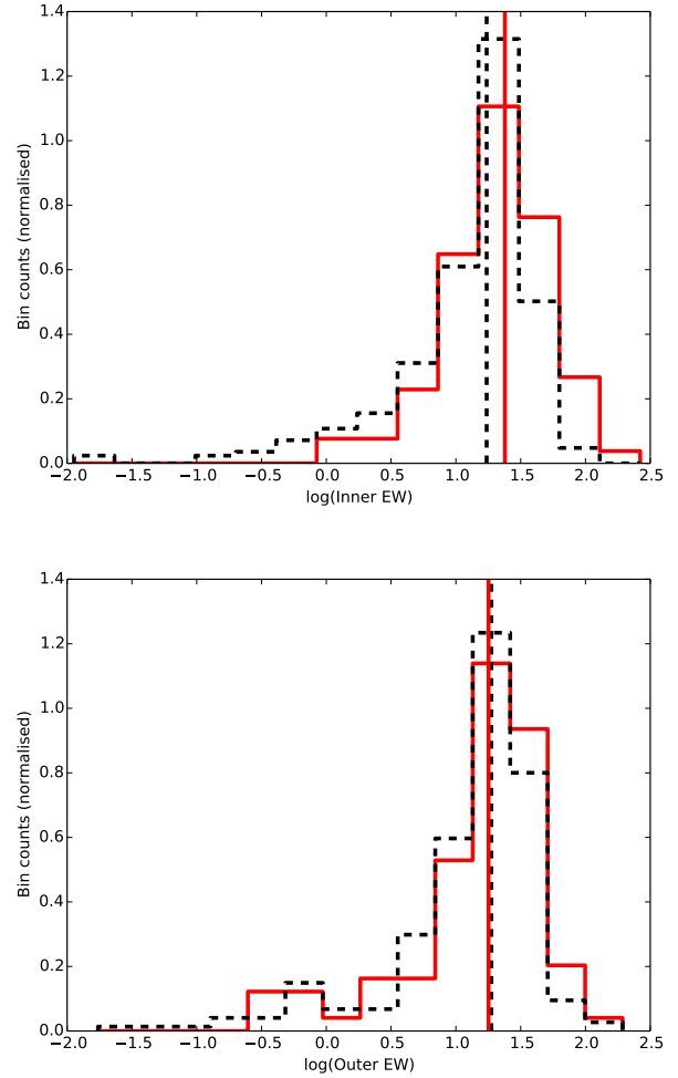
Figure 21. We show normalised histograms of the equivalent width within half an effective radius (top) and outside this range (bottom) for kinematically asymmetric (red) and normal (black, dashed) galaxies. The median equivalent widths in each case are shown for asymmetric (red, solid) and normal (black, dashed) galaxies. The medians are the same for the \log(\text{outer EW}) , and there is a marginally significant offset for the \log(\text{inner EW}) . A two-sample Kolmogorov-Smirnov test of the distributions of \log(\text{inner EW}) yields a p-value of 0.0090, indicating that the distributions of \log(\text{inner EW}) for kinematically asymmetric and normal galaxies are statistically dissimilar, whereas this is not the case for \log(\text{outer EW}) .
