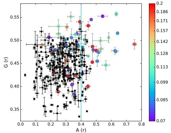
Figure 13. We show the A - G plane for kinematically normal (black) and kinematically asymmetric (coloured) galaxies. Errors are 1-\sigma errors on both axes. As anticipated, only a weak relation emerges between asymmetry and plane location. The blue line indicates A \sim 0.4 , below which the relationship between A and asymmetry becomes significantly weaker.
