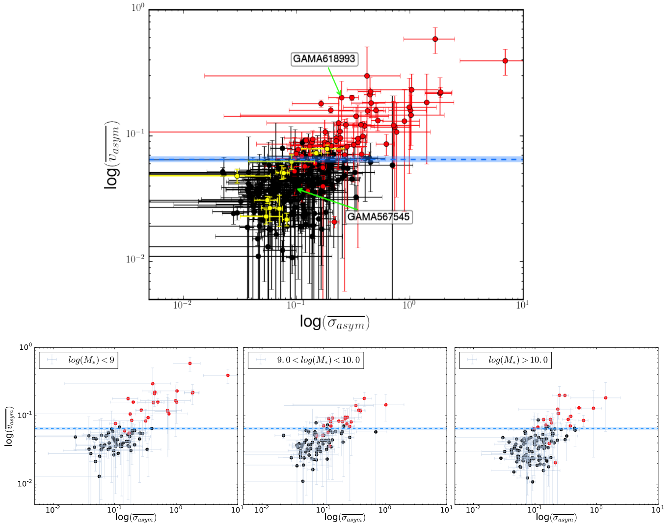
Figure 8. These plots summarise the results of kinemetry for the 360 galaxies in our sample (top) and three stellar mass bins (bottom row). The median kinematic asymmetries for both velocity and velocity dispersion across fitted ellipse radii are normalised over the rotational velocity and plotted against each other. The sample was visually classified morphologically (using the SDSS DR10 images), with visually asymmetric galaxies shown here in red, and ‘possibly asymmetric’ galaxies in yellow. We show the \bar{v}_{asym} cutoff for kinematic asymmetry derived in the text (blue, dashed line). The two example galaxies from Fig. 6, GAMA567545 (the normal galaxy) and GAMA618993 (the asymmetric galaxy) are indicated by the green arrows, for reference.
