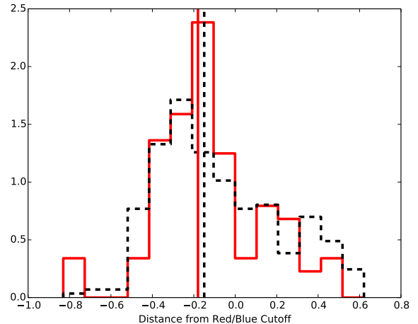
Figure 17. We show a normalised histogram of distance (in colour space) from red/blue cutoff for kinematically asymmetric (red) and normal (black, dashed) galaxies. The median offset for each distribution is shown by the vertical lines. There is no significant offset between the kinematically asymmetric and normal medians, indicating that, independent of mass, there is no relationship between colour and \overline{v_{asym}} .
