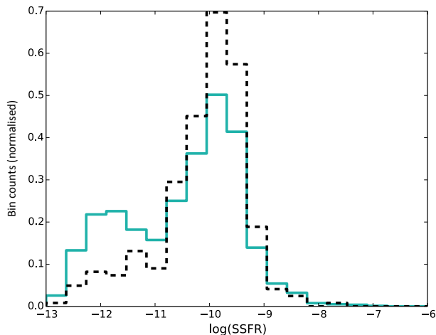
Figure 5. We show a normalised histogram of the specific SFR in the SAMI Galaxy Survey sample (blue) and the sample used in this work (black, dashed). The data used were taken from the GAMA Data Release 2 catalogues SpecLineSFR (Hill et al. 2011) and StellarMasses (Taylor et al. 2011).
