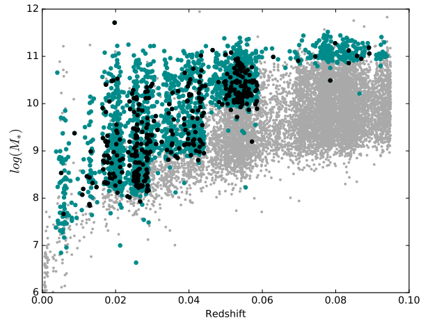
Figure 3. We show redshift and stellar mass for the GAMA Survey sample (grey points), SAMI Galaxy Survey sample (blue points) and our sample (black dots). Our sample is evenly distributed within the main SAMI Galaxy Survey sample. The data used were taken from the GAMA Data Release 2 catalogues StellarMasses (Taylor et al. 2011) and SpecLineSFR (Hopkins et al. 2013).
